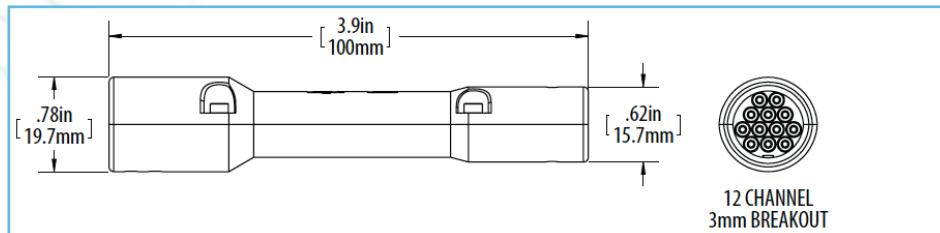
Tac-Grip Metal Breakout Kit Dimensions
